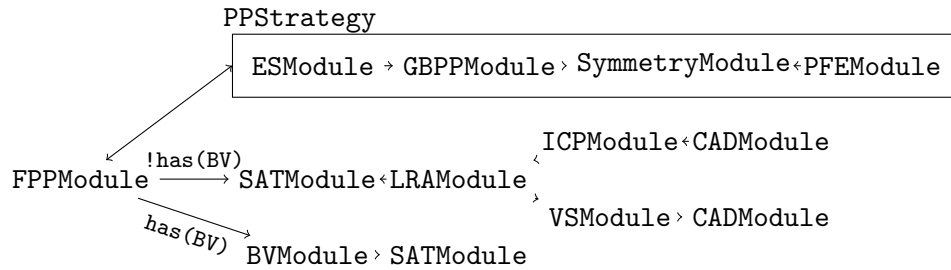
Figure 1: An example SMT-RAT strategy
