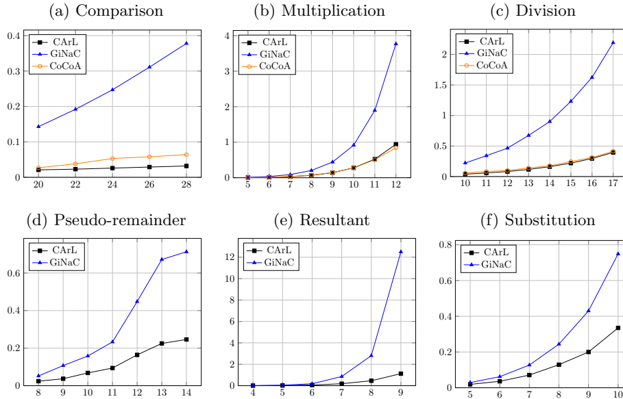
Figure 2: Experimental results for polynomial computations
